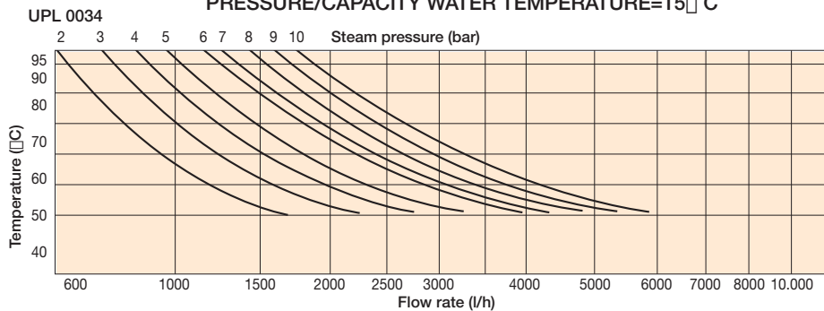
PRESSURE/CAPACITY WATER TEMPERATURE=15° C
